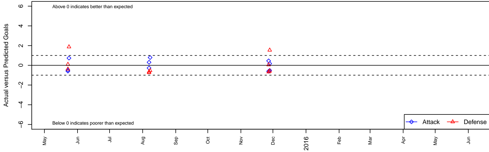
LA Galaxy Bakersfield B97 Dots are actual minus expected GF (blue circles) and GA (red triangles). Blue line is smoothed change in attack strength. Red is smoothed change in defense strength.
